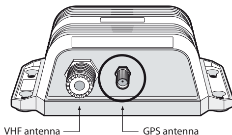
Figure 8 Position of the GPS antenna connector
