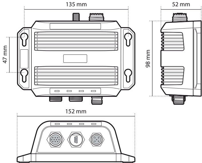
Figure 5 AIS transceiver dimensions
