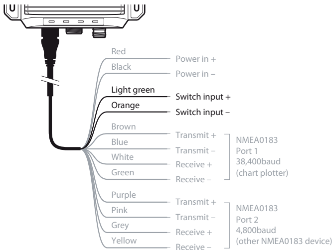
Figure 10 Connecting an external switch
