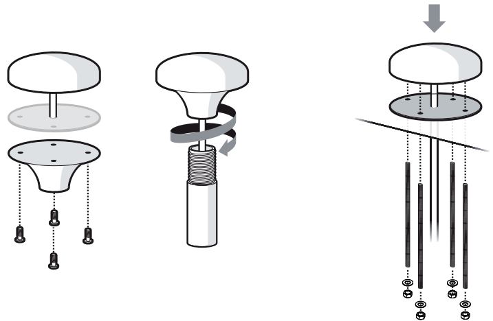
Figure 7 GPS antenna mounting
