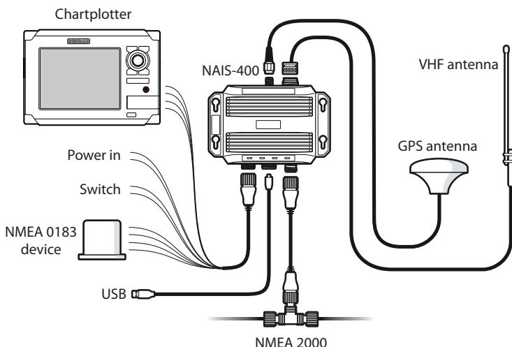
Figure 4 Typical installation configuration
