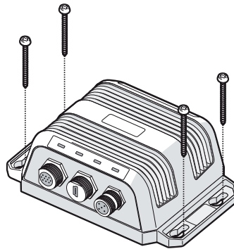
Figure 6 AIS transceiver mounting
