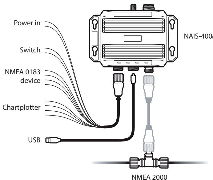
Figure 3 Electrical connections to the AIS transceiver
