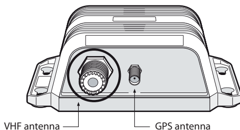
Figure 9 Position of the VHF antenna connector
