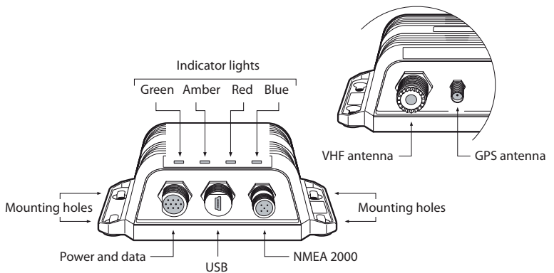
Figure 2 AIS transceiver overview
